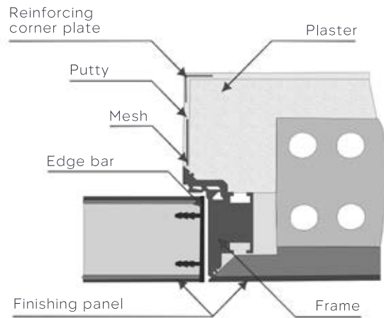
PANEL LEAF OUTSIDE OPENING
