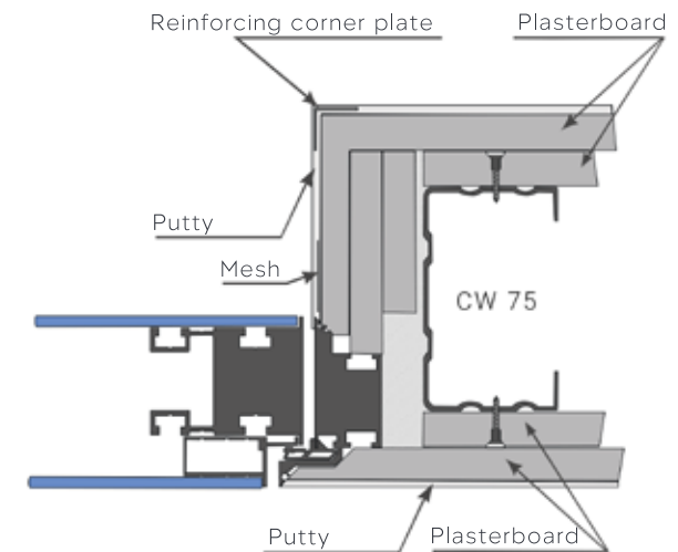
LEAF - ALUMINIUM CARCASS INSIDE OPENING
