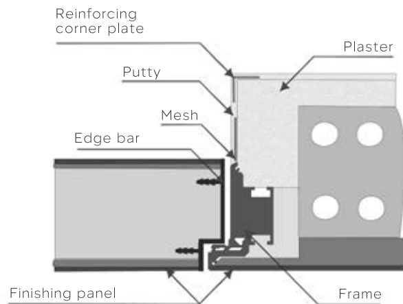
PANEL LEAF INSIDE OPENING
