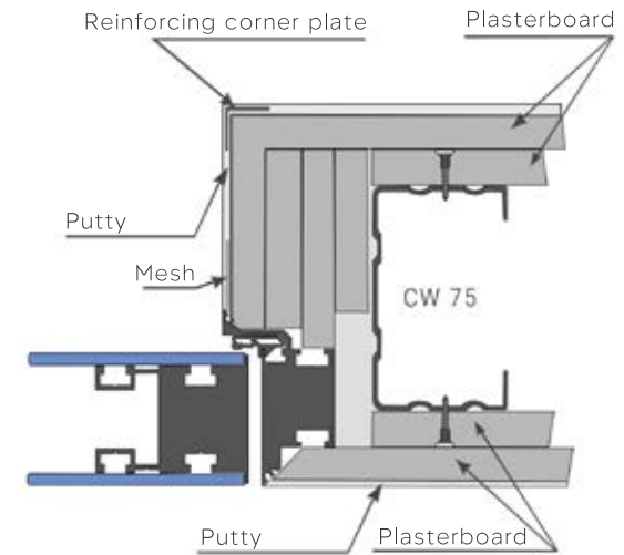
LEAF - ALUMINIUM CARCASS OUTSIDE OPENING
